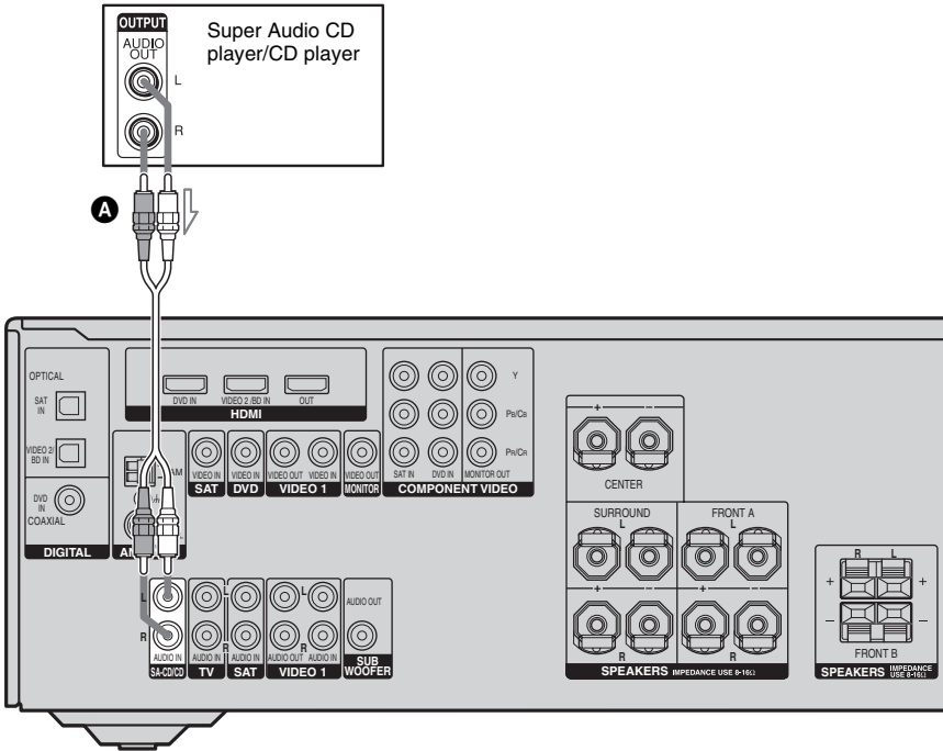
A Audio cord (not supplied)
